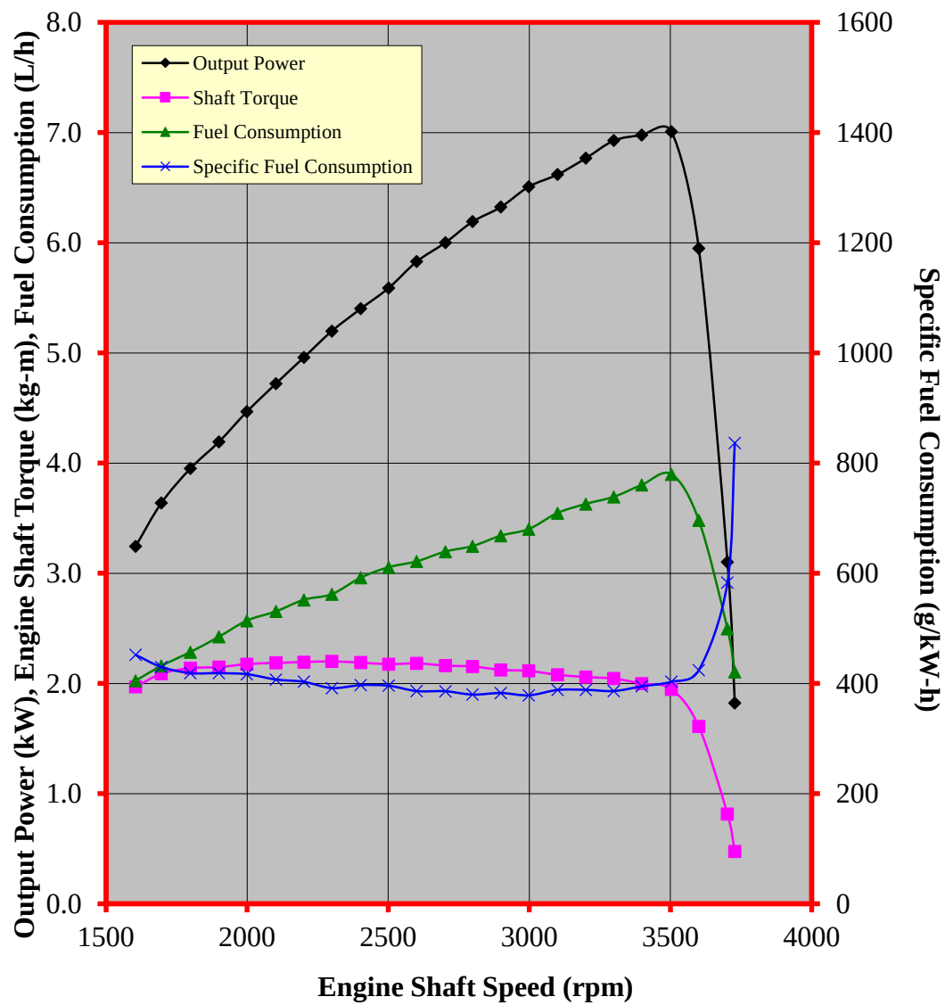
Figure 3. Performance characteristic curves of the HONDA GX390H1 QHP1 gasoline engine
