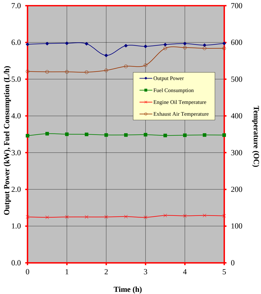
Figure 4. Performance characteristic curves during the continuous running test of the HONDA GX390H1 QHP1 gasoline engine
