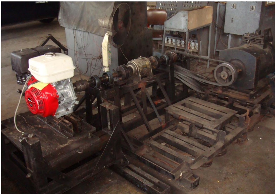
Figure 2. Test set-up of the HONDA GX390H1 QHP1 Gasoline Engine
